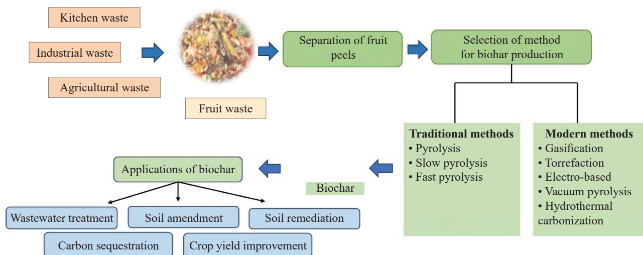
Figure 4 Fruit peel waste utilization for producing biochar and its applications [75, 84]
